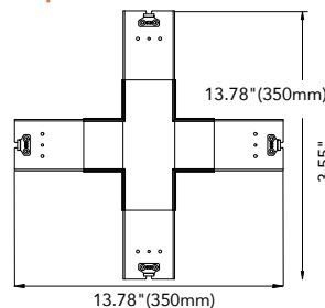
XLS(X-Shape)
