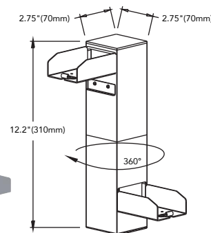
360° Rotable
