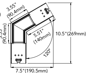
CLS(120°L-Shape)
