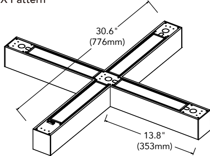
X Pattern
