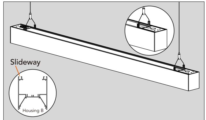
Housing B
