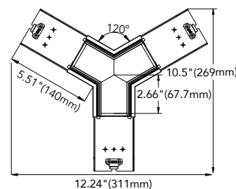
YLS(Y-Shape)
