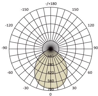
Commercial-WL-DL04IN15W-930 Commercial-WL-DL/4"/15W/RA90/3000K
