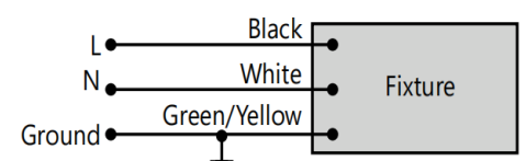
Wiring Diagram Fig. C2
