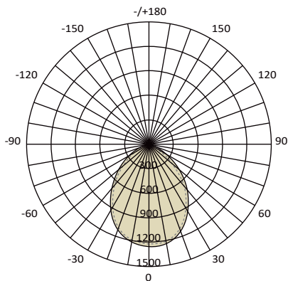
Commercial-WL-DL06IN24W-930 Commercial-WL-DL/6"/24W/RA90/3000K
