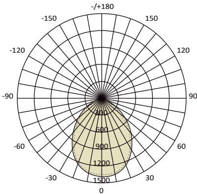
Commercial-WL-DL08IN30W-930 Commercial-WL-DL/8"/30W/RA90/3000K
