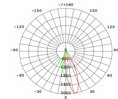
Cleaver G3-WL-3COV
