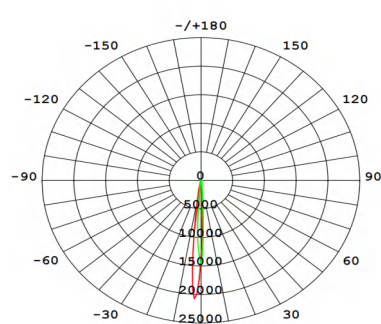
Cleaver G3-WL-3COV
