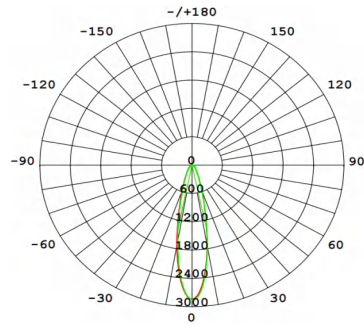
Cleaver G3-WL-3COV
