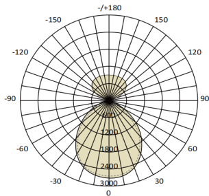
Sense-199-8FT100W-840-WH-30 Sense-199-8'/100W/RA80/4000K/White/Up30%,Down 70%
