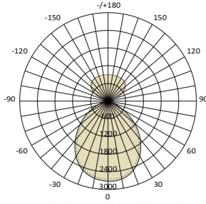
Sense-199-4FT50W-840-WH-30 Sense-199-4'/50W/RA80/4000K/White/Up30%,Down 70%
