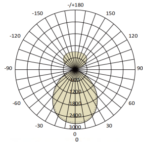
Sense-199-2FT25W-840-WH30 Sense-199-2'/25W/RA80/4000K/White/Up30%,Down 70%
