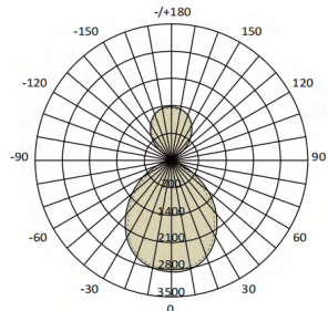
Sense-198-8FT100W-840-WH-30 Sense-198/8'/100W/RA80/4000K/White/Up30%,Down 70%
