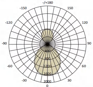
Sense-198-4FT50W-840-WH-30 Sense-198/4'/50W/RA80/4000K/White/Up30%,Down 70%
