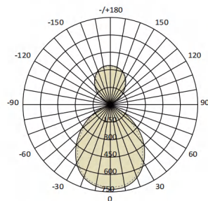
Sense-198-2FT25W-840-WH30 Sense-198/2'/25W/RA80/4000K/White/Up30%,Down 70%
