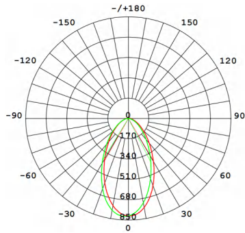
CLEAVER G5 COVE LIGHT-WL-5COV 1FT/10W/RA90/60°/3500K/White
