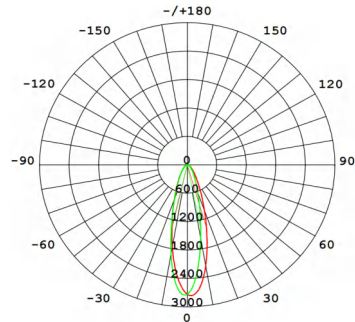
CLEAVER G5 COVE LIGHT-WL-5COV 1FT/10W/RA90/25°/3500K/White
