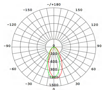
CLEAVER G5 COVE LIGHT-WL-5COV 1FT/10W/RA90/45°/3500K/White
