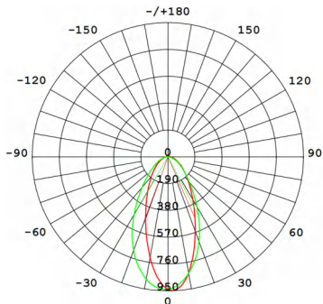
CLEAVER G5 COVE LIGHT-WL-5COV 1FT/10W/RA90/45°×60°/3500K/White
