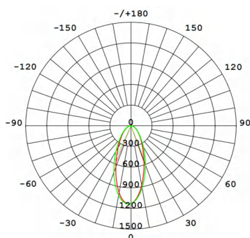
CLEAVER G5 COVE LIGHT-WL-5COV 1FT/10W/RA90/40°×45°/3500K/White
