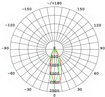
CLEAVER G5 COVE LIGHT-WL-5COV 1FT/10W/RA90/35°/4000K/White
